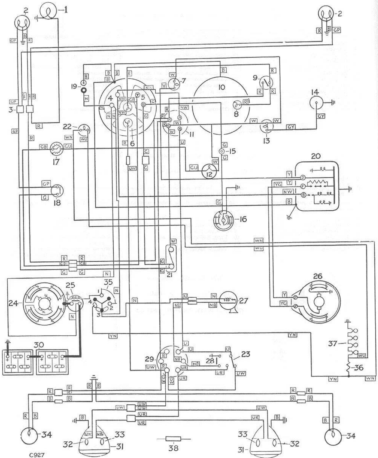
Fig. P-9—Wiring diagram, Diesel models.
