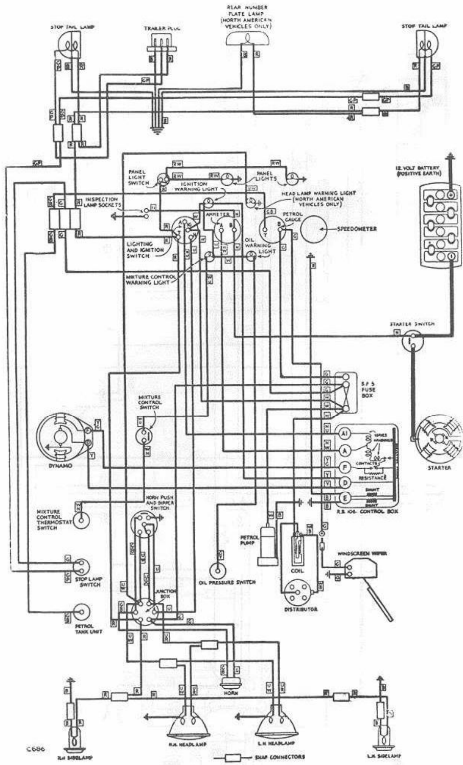
Fig. P-5—Wiring diagram, late 1951, 1952 and 1953 models
